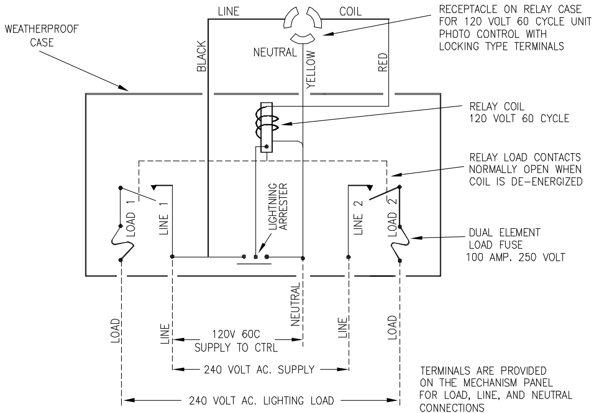
CONNECTIONS FOR TYPE MR-YG 2POLE 100 AMPERE RELAY.
