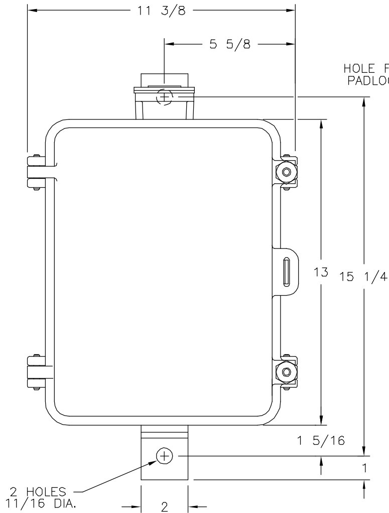
CAST ALUMINUM WEATHERPROOF CASE WITH BRACKET, CAST ALUMINUM RECEPTACLE HOUSING FOR 2 POLE 100A RELAYS.
